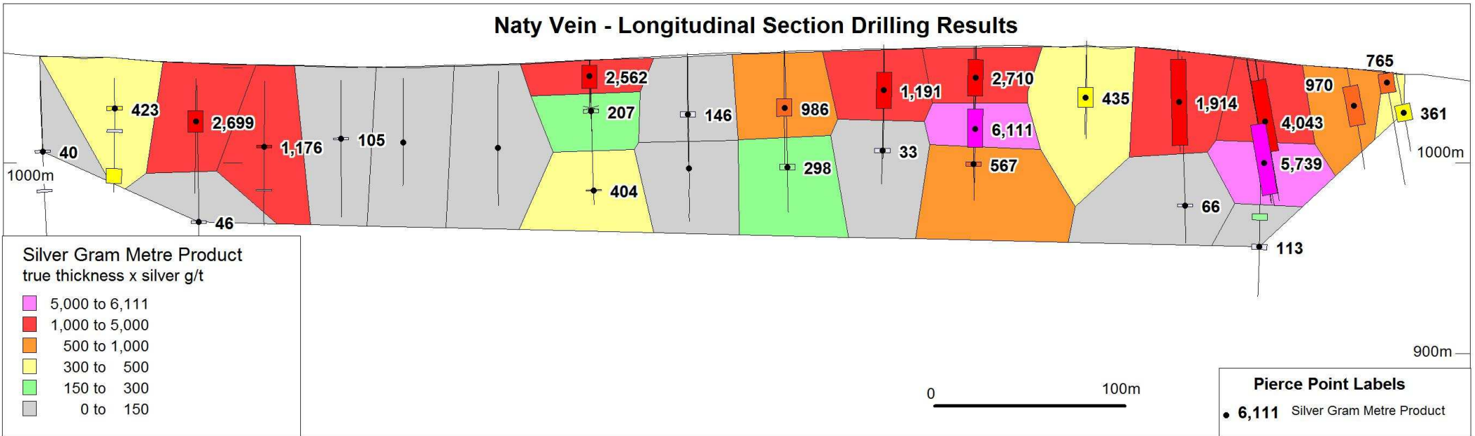
Mirasol Resources. Virginia Silver Project, Natty Vein Drill Results. Figure 4a. June, 2012
