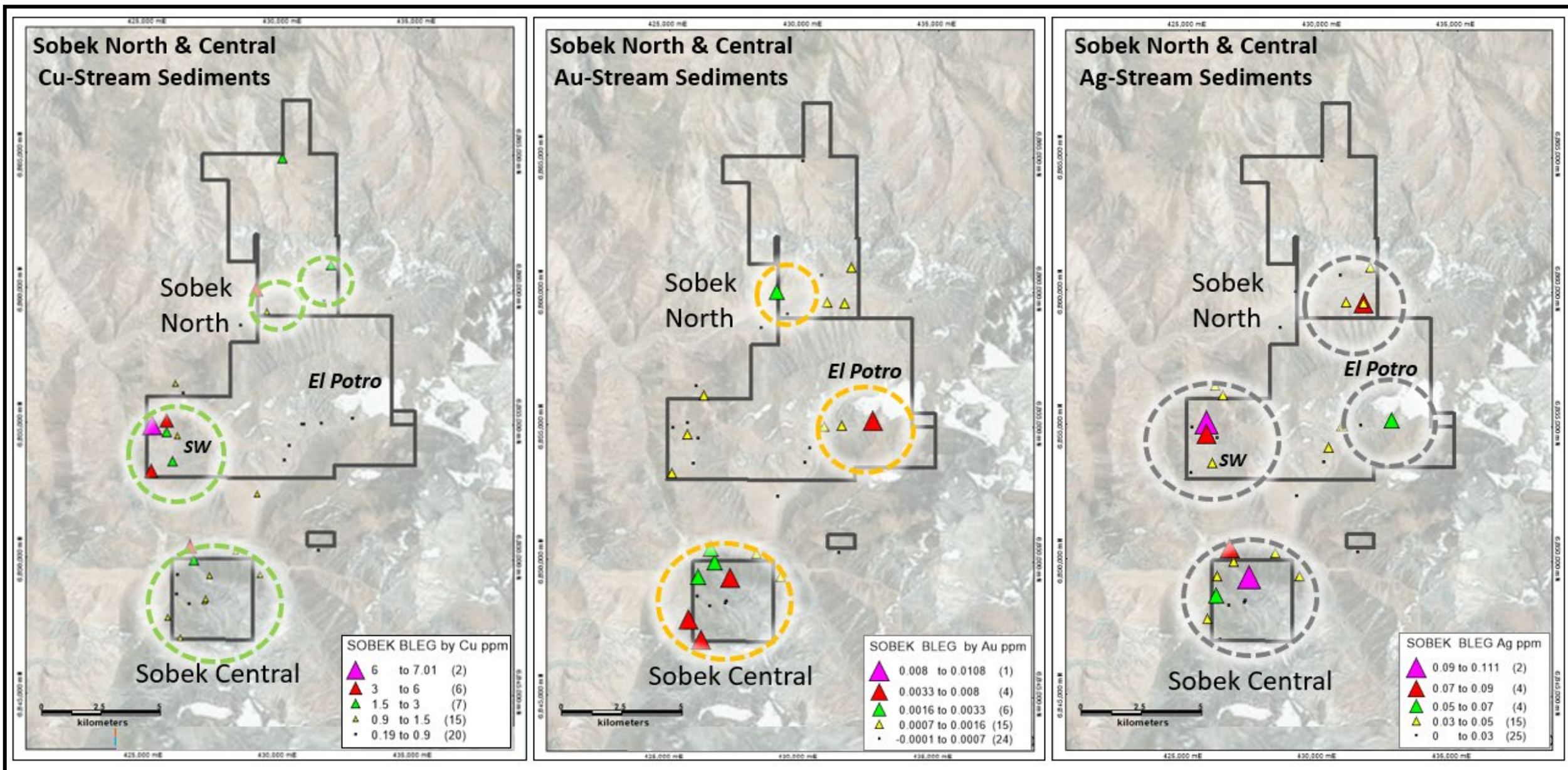
Figure 3: Sobek Central and Sobek North - Stream Sediment Sample Anomalies
