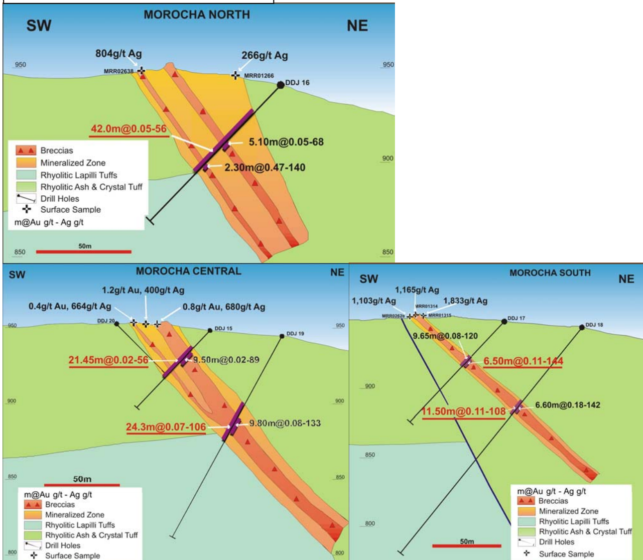
Figure 7: La Morocha cross sections
