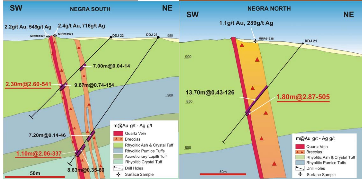
Figures 5: La Negra cross sections
