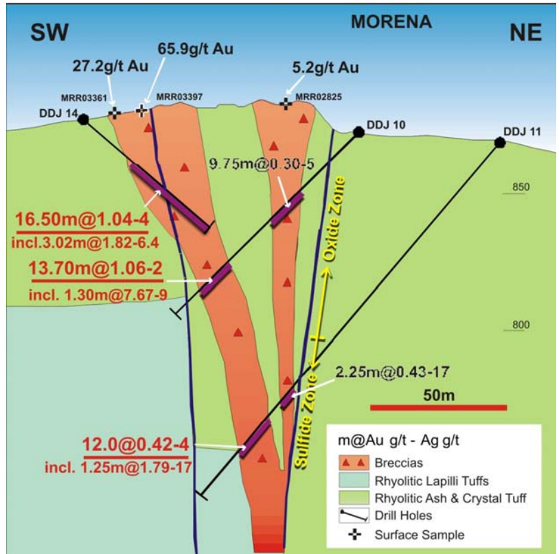
Figure 2: La Morena cross section
