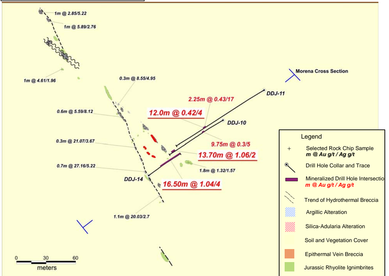
Figure 3: La Morena surface map
