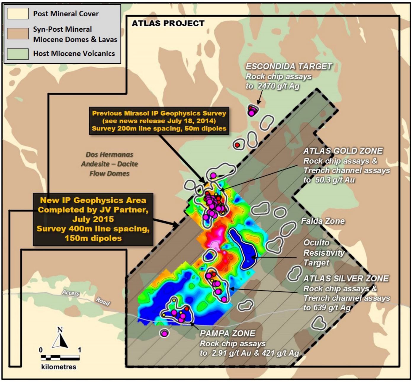
Figure 1: Gorbea Gold Belt Joint Venture: Atlas Pole Dipole Survey. July 2015.
